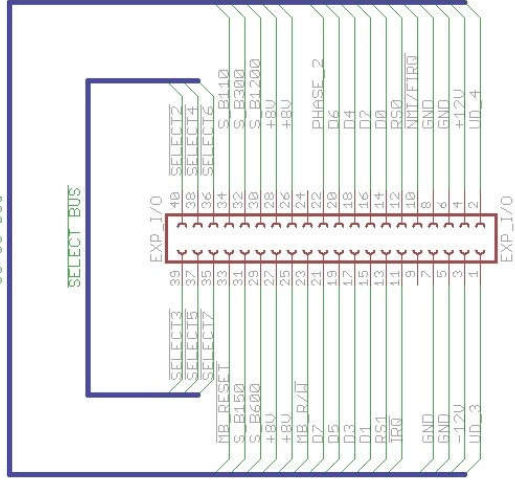
SS-30 BUS
