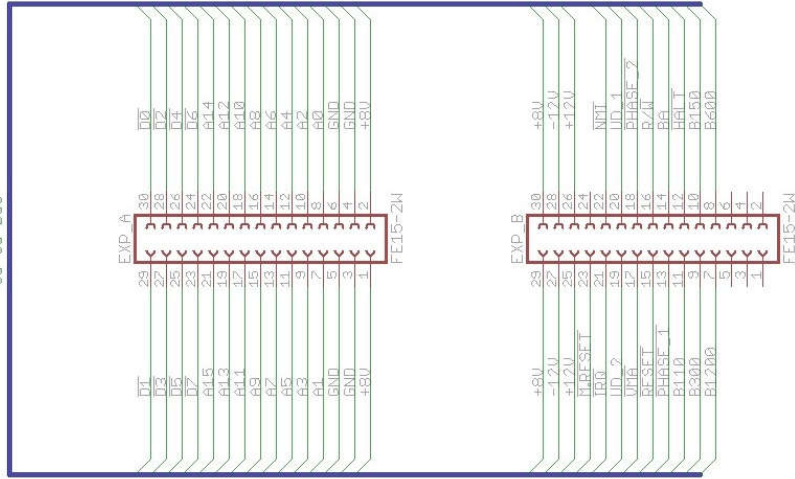
SS-50 BUS
