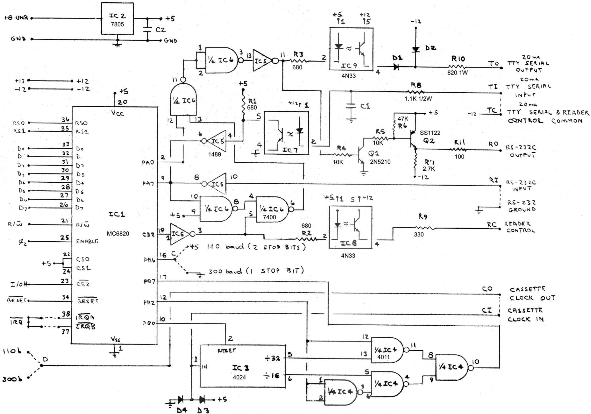
Schematic - MP-C Serial Control Interface
